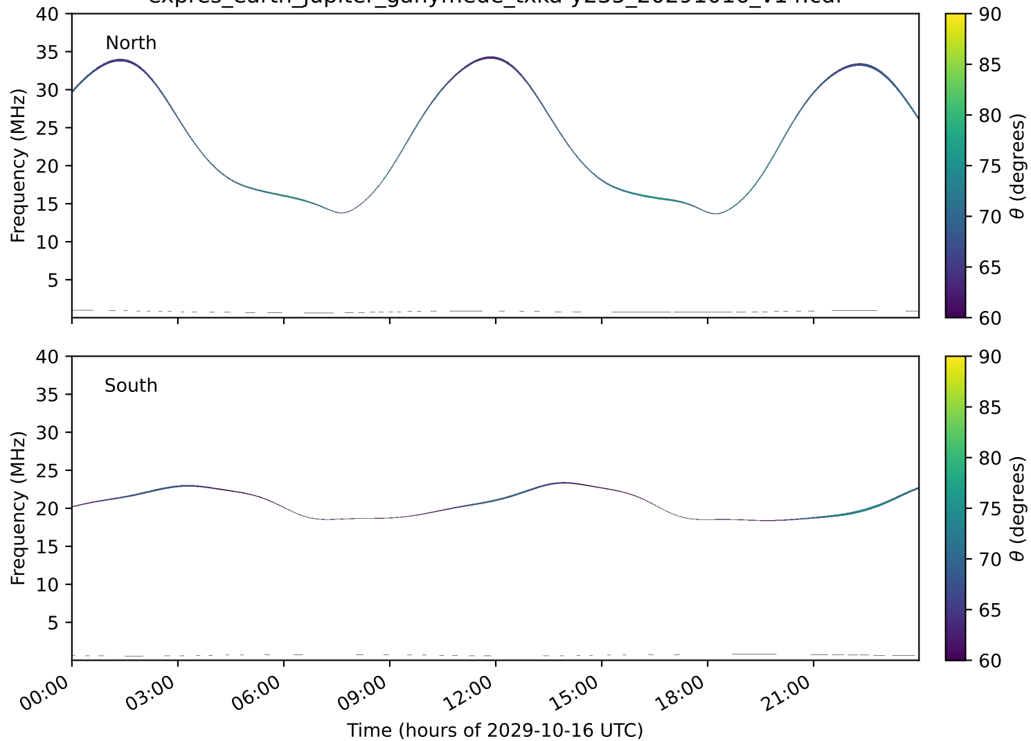
expres_earth_jupiter_ganymede_txka-y235_20291016_v14.cdf
