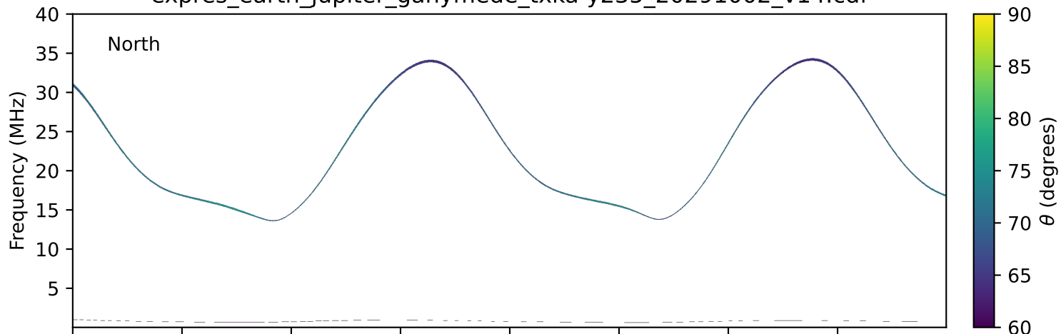
expres_earth_jupiter_ganymede_txka-y235_20291002_v14.cdf
