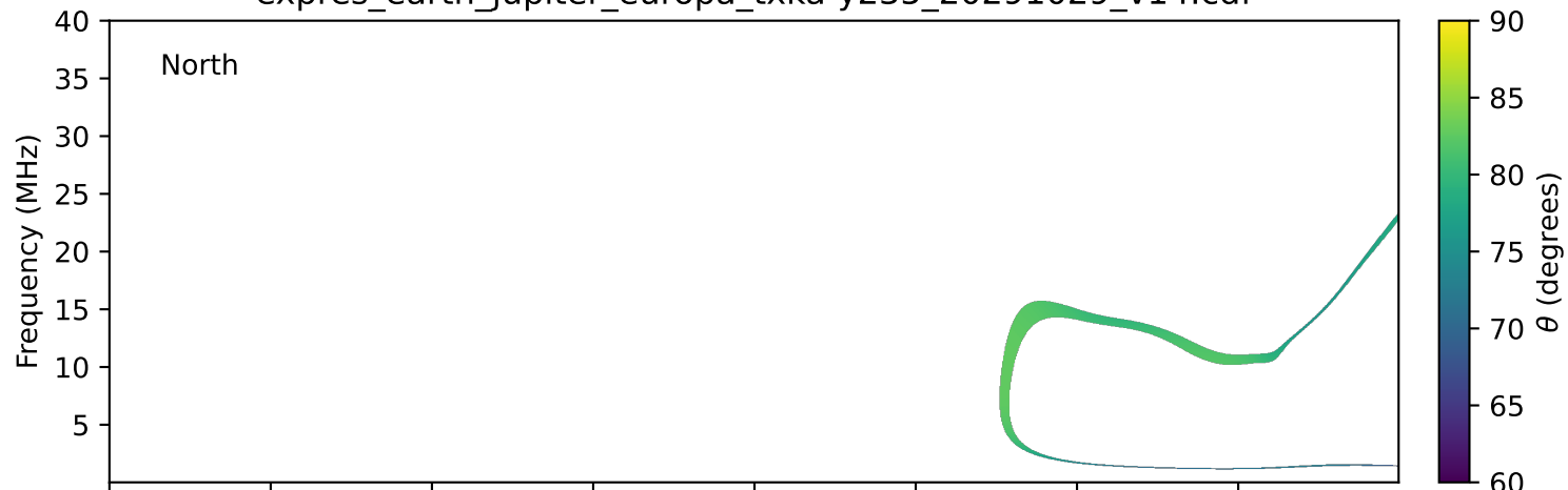
expres_earth_jupiter_europa_txka-y235_20291029_v14.cdf
