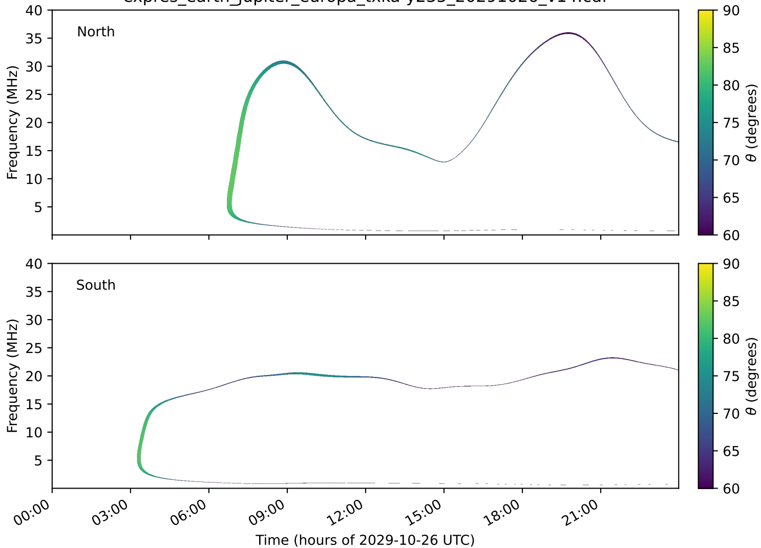
expres_earth_jupiter_europa_txka-y235_20291026_v14.cdf
