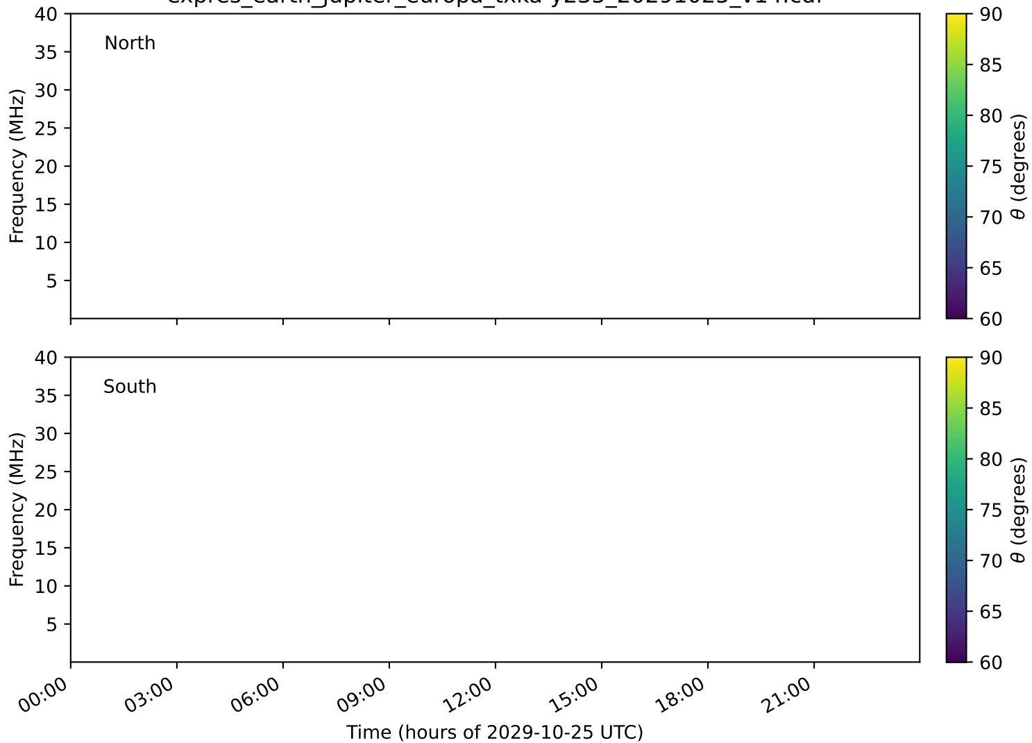
expres_earth_jupiter_europa_txka-y235_20291025_v14.cdf
