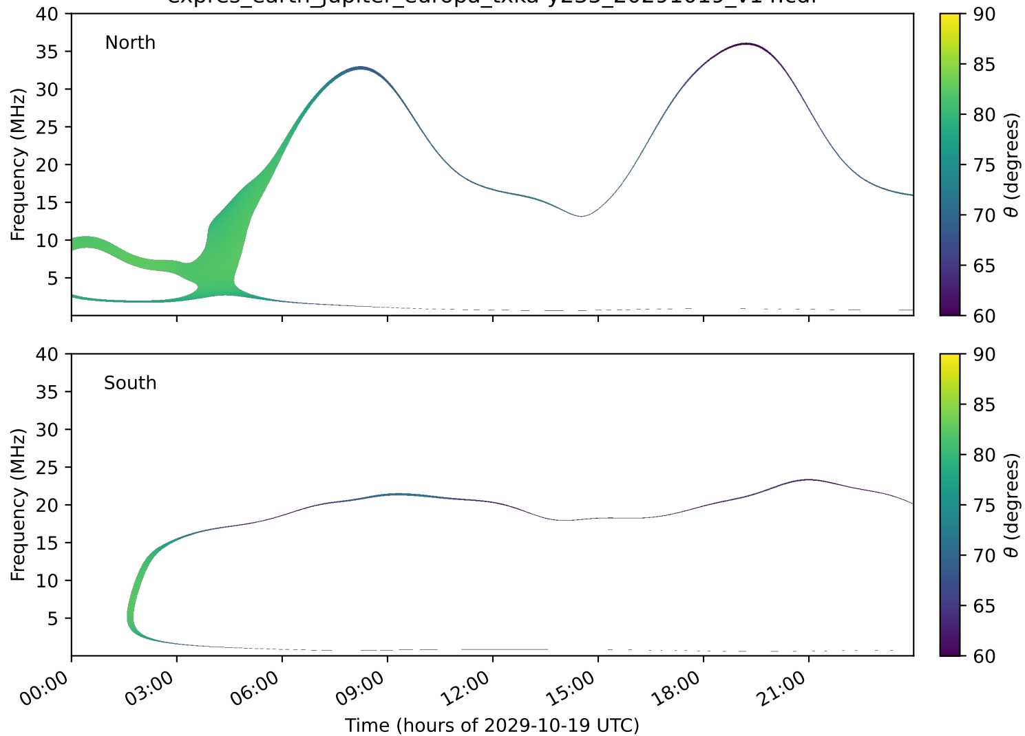
expres_earth_jupiter_europa_txka-y235_20291019_v14.cdf
