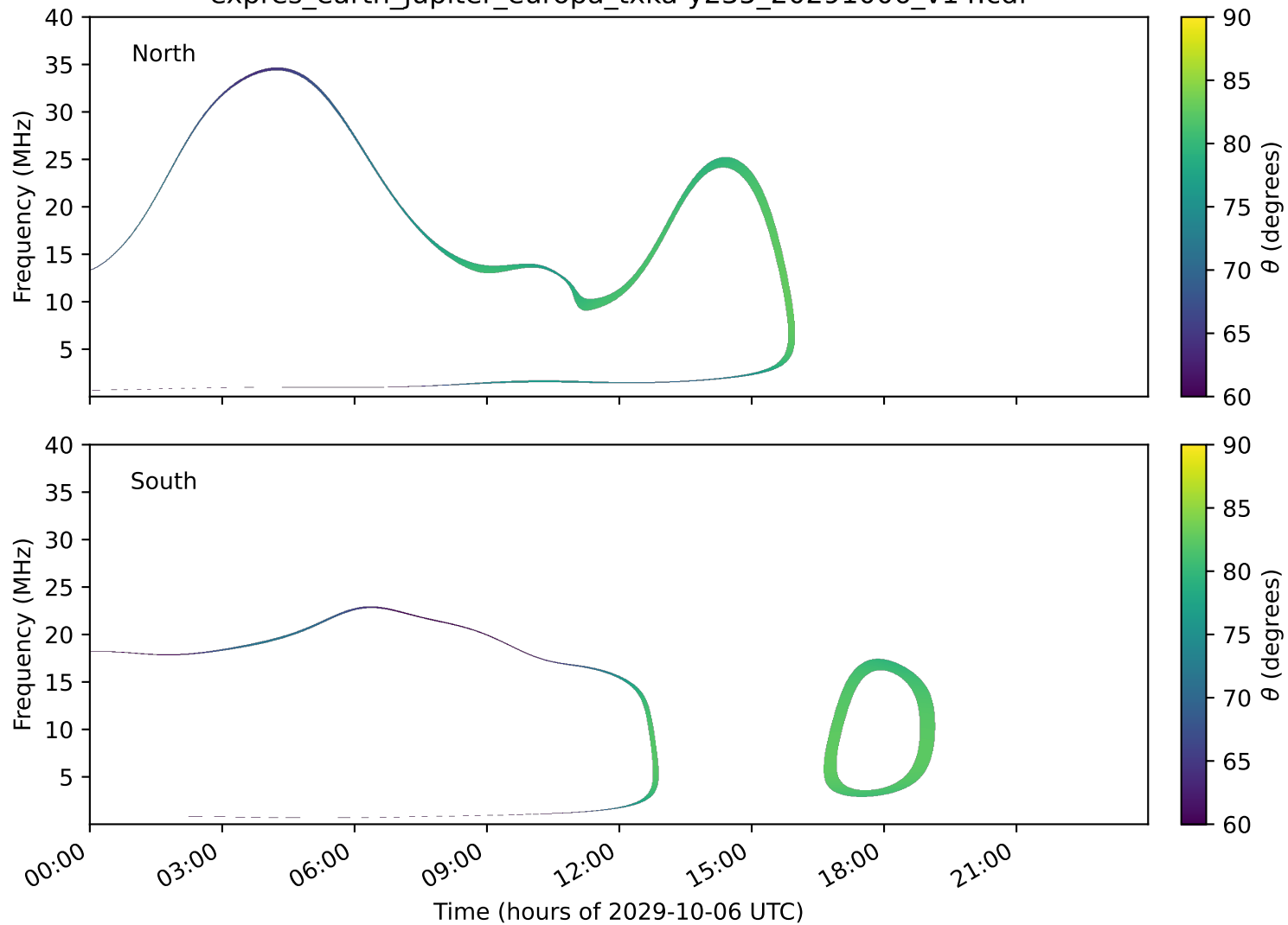
expres_earth_jupiter_europa_txka-y235_20291006_v14.cdf
