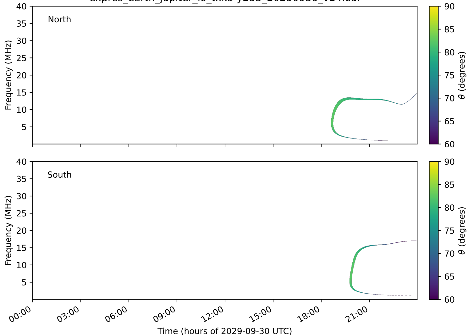
expres_earth_jupiter_io_txka-y235_20290930_v14.cdf
