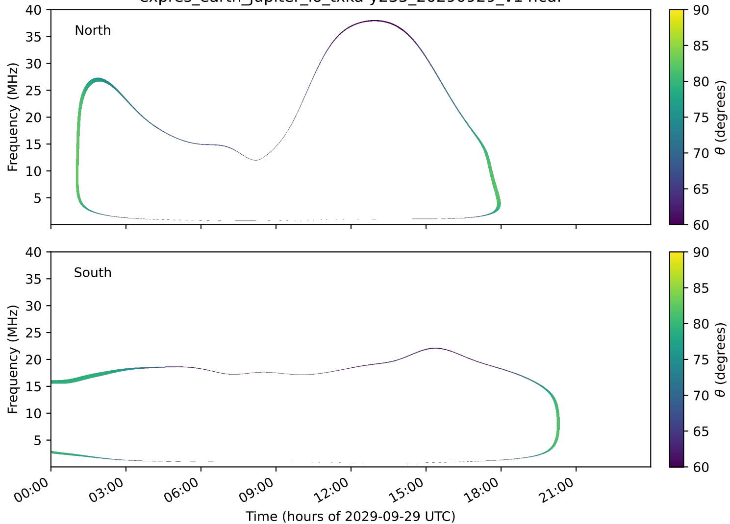
expres_earth_jupiter_io_txka-y235_20290929_v14.cdf
