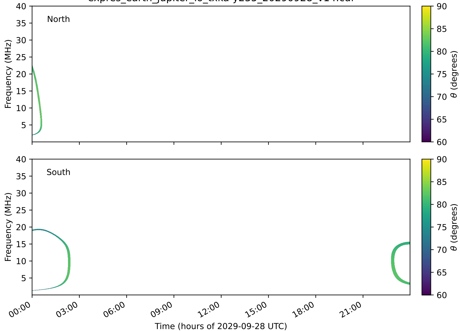
expres_earth_jupiter_io_txka-y235_20290928_v14.cdf
