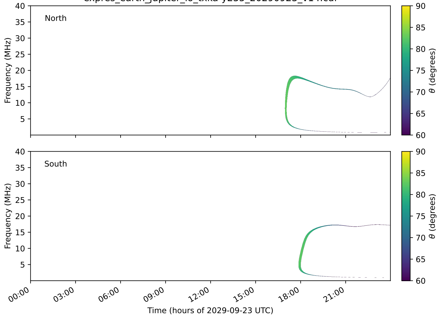
expres_earth_jupiter_io_txka-y235_20290923_v14.cdf
