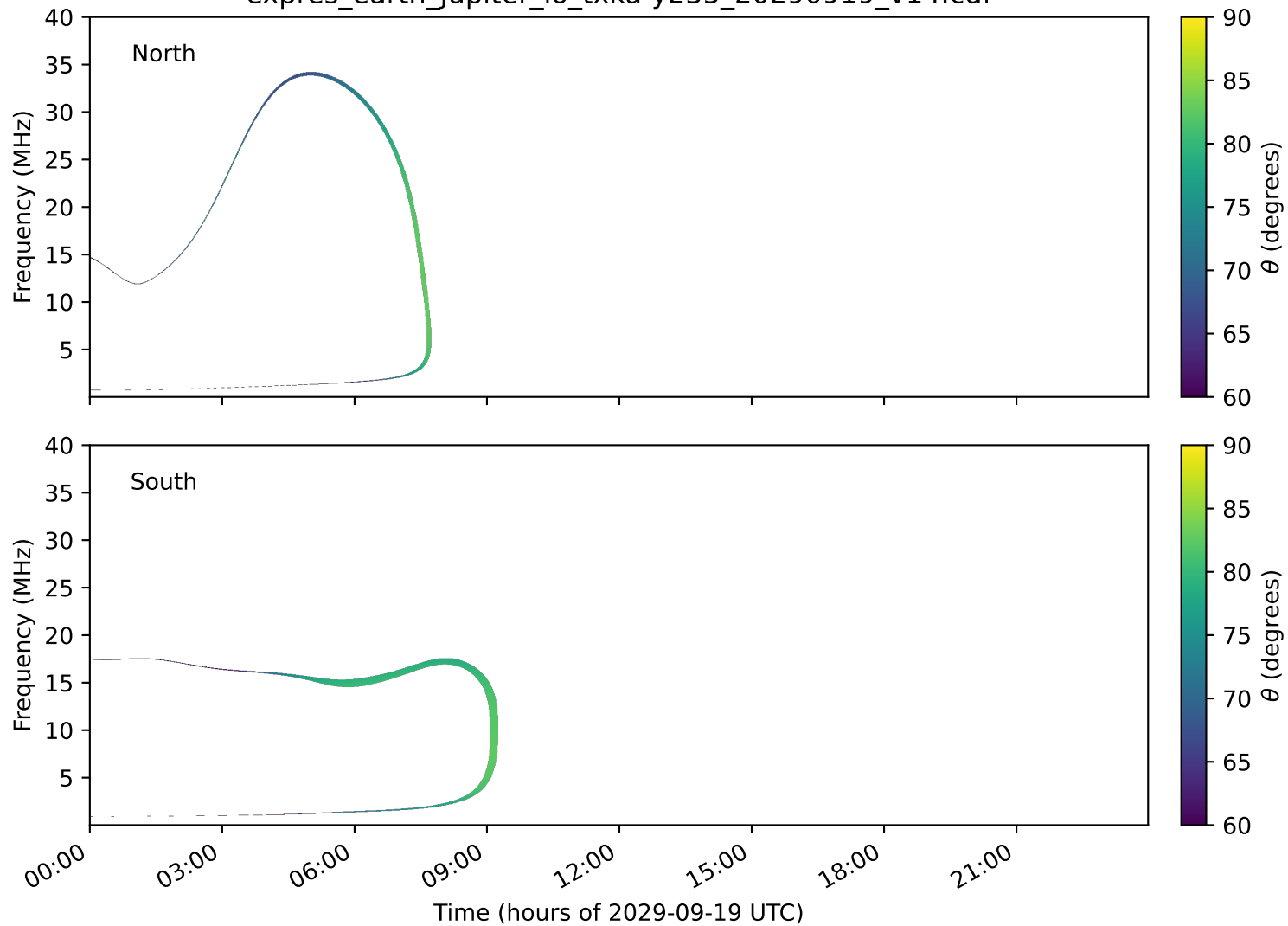
expres_earth_jupiter_io_txka-y235_20290919_v14.cdf
