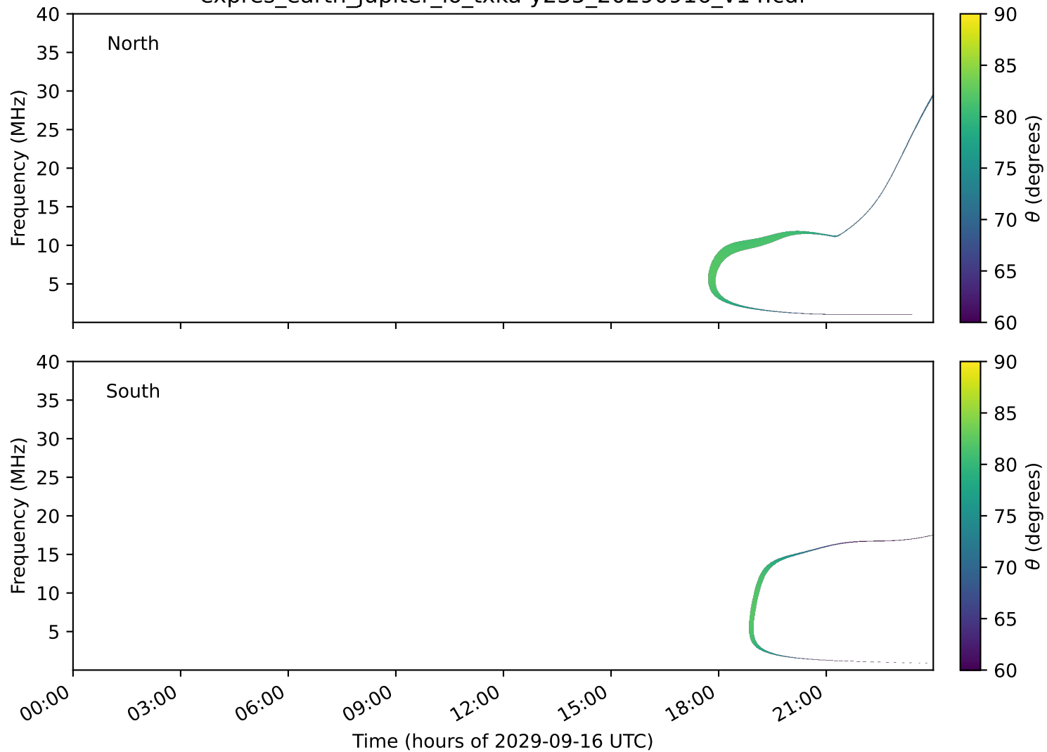
expres_earth_jupiter_io_txka-y235_20290916_v14.cdf
