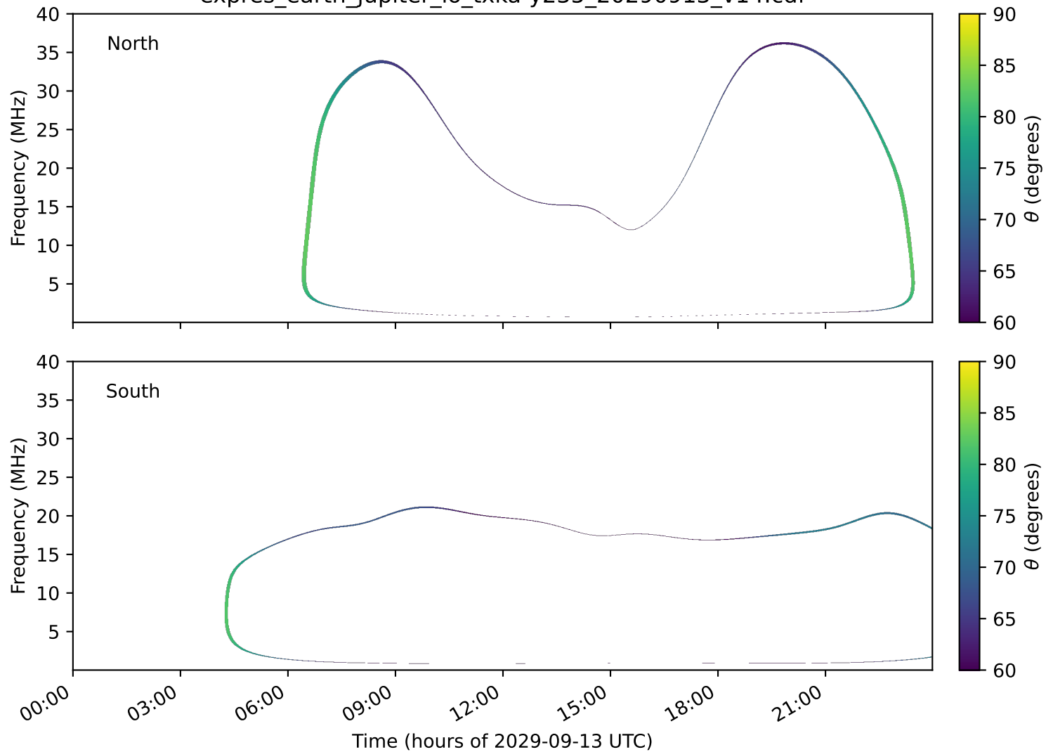
expres_earth_jupiter_io_txka-y235_20290913_v14.cdf
