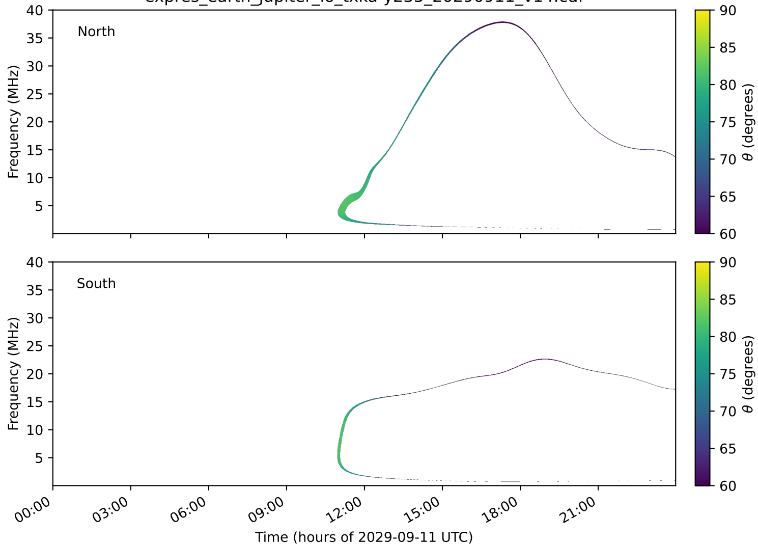
expres_earth_jupiter_io_txka-y235_20290911_v14.cdf
