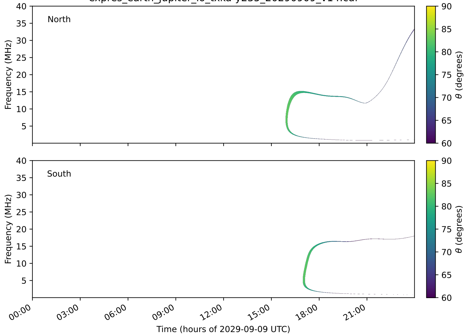
expres_earth_jupiter_io_txka-y235_20290909_v14.cdf
