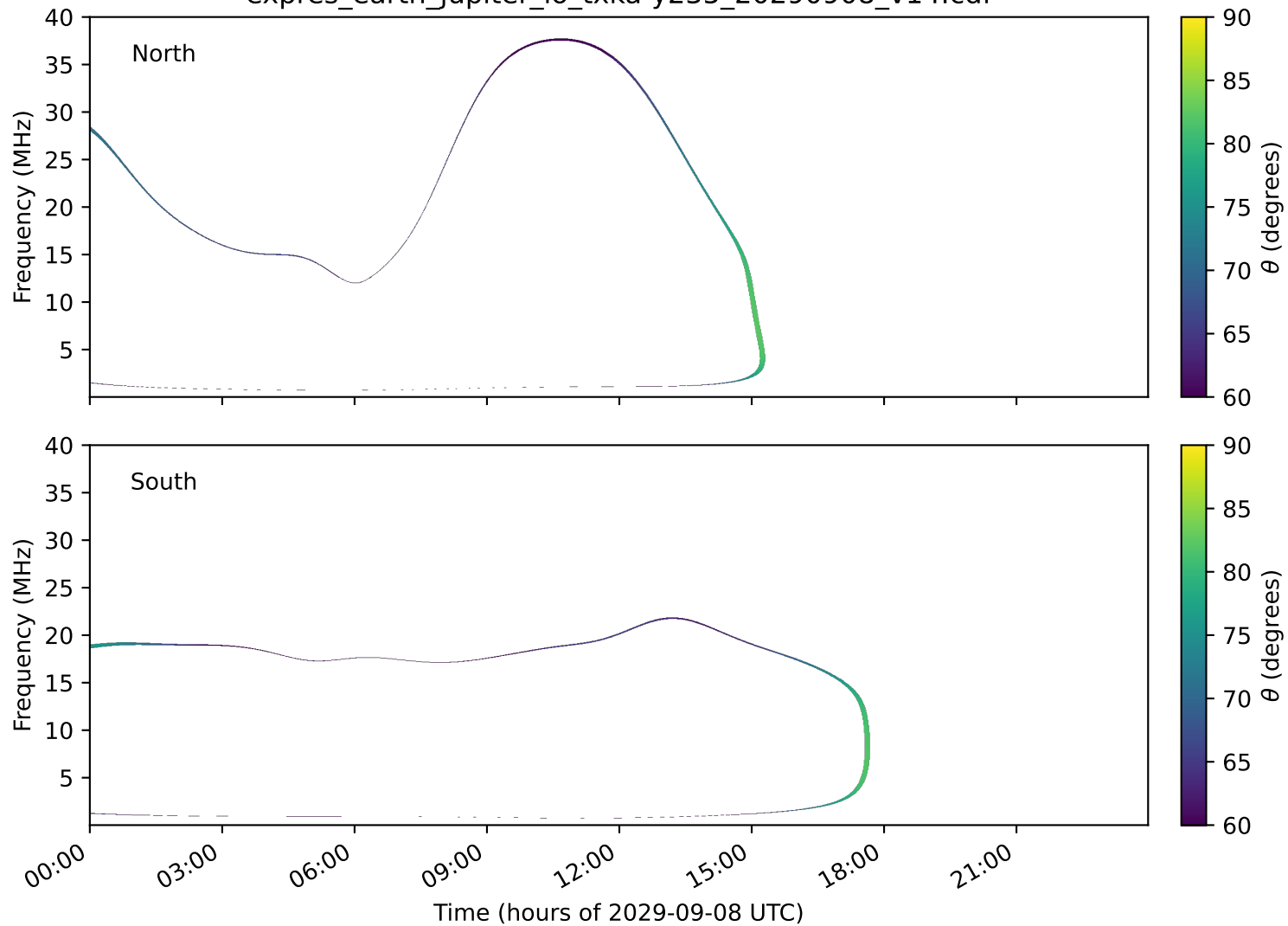
expres_earth_jupiter_io_txka-y235_20290908_v14.cdf
