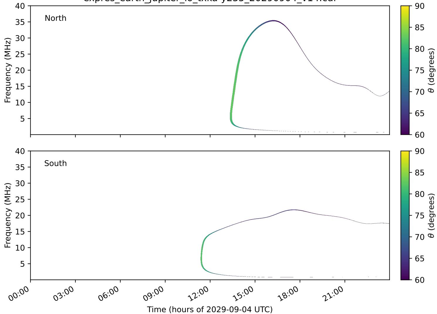
expres_earth_jupiter_io_txka-y235_20290904_v14.cdf
