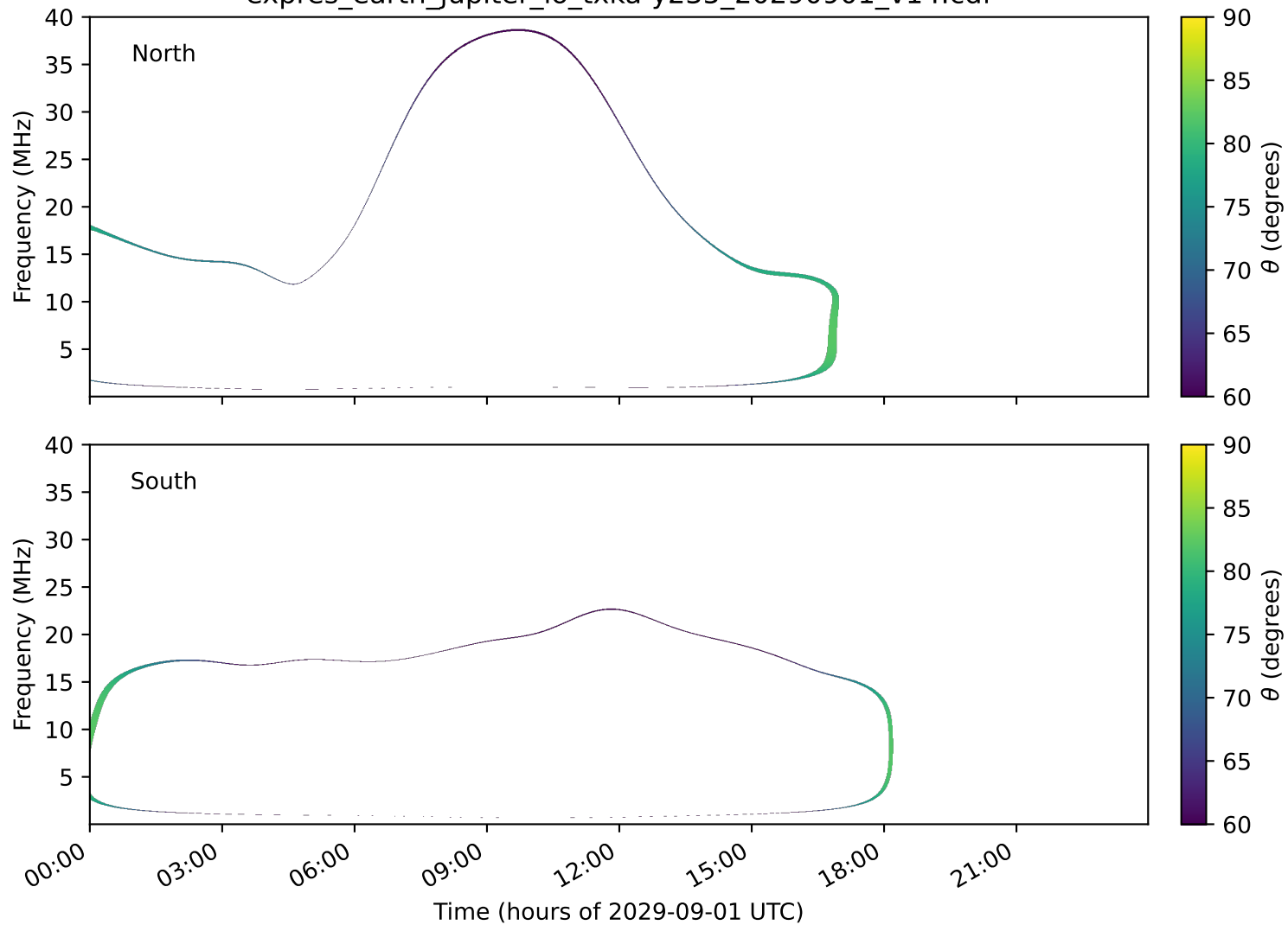
expres_earth_jupiter_io_txka-y235_20290901_v14.cdf
