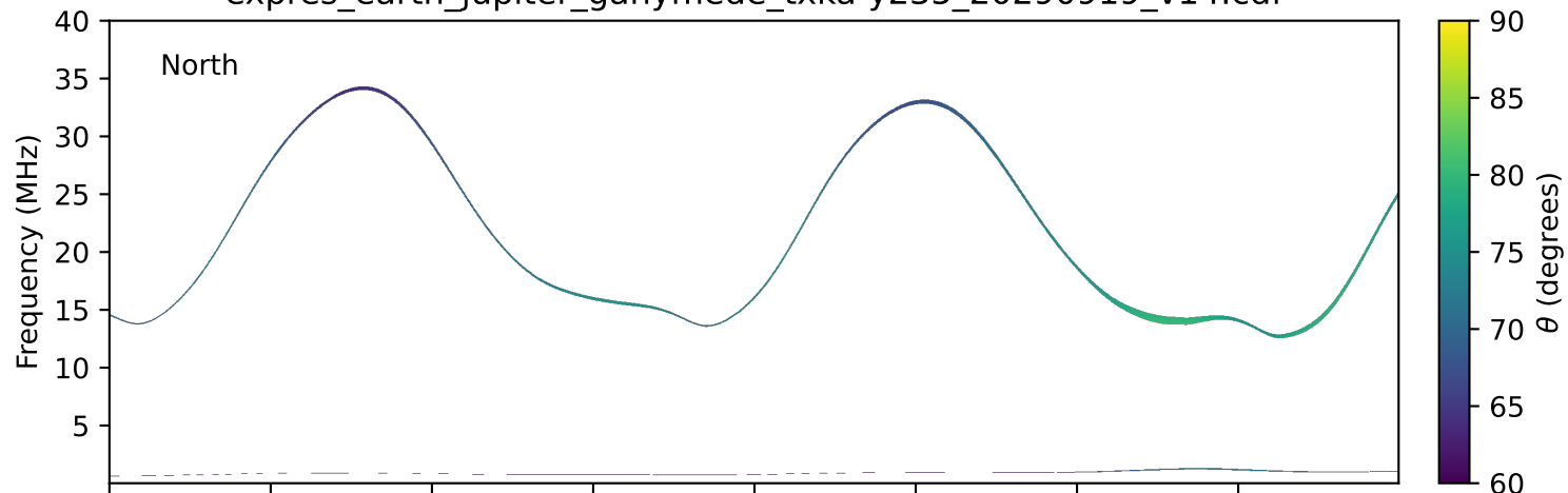
expres_earth_jupiter_ganymede_txka-y235_20290919_v14.cdf
