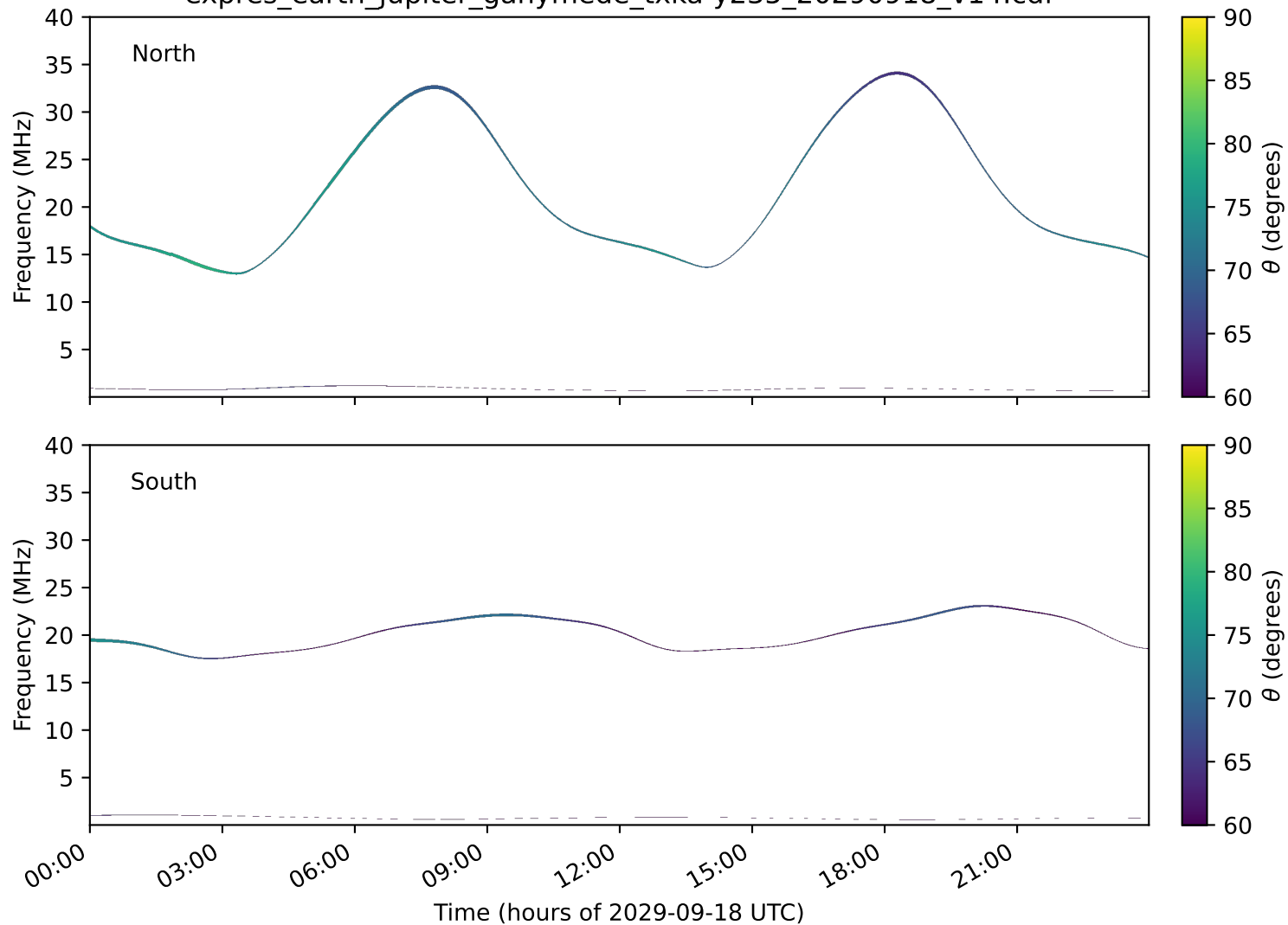
expres_earth_jupiter_ganymede_txka-y235_20290918_v14.cdf
