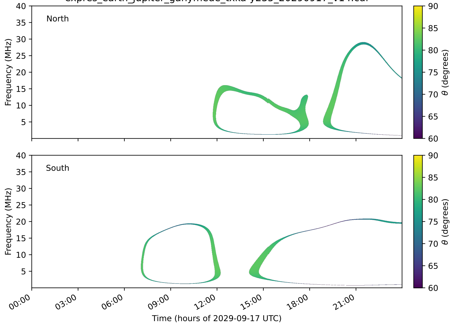
expres_earth_jupiter_ganymede_txka-y235_20290917_v14.cdf
