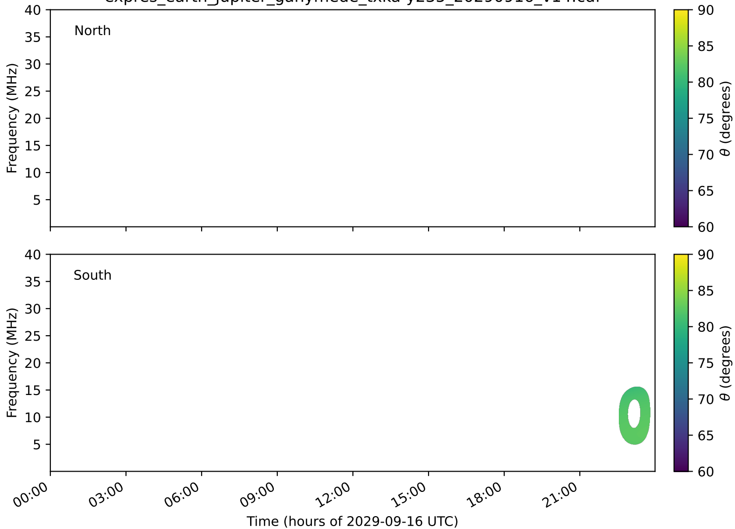
expres_earth_jupiter_ganymede_txka-y235_20290916_v14.cdf
