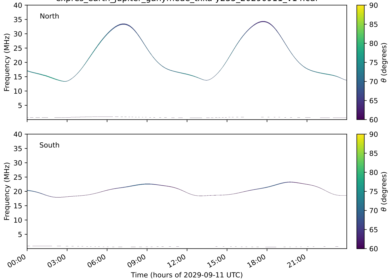
expres_earth_jupiter_ganymede_txka-y235_20290911_v14.cdf
