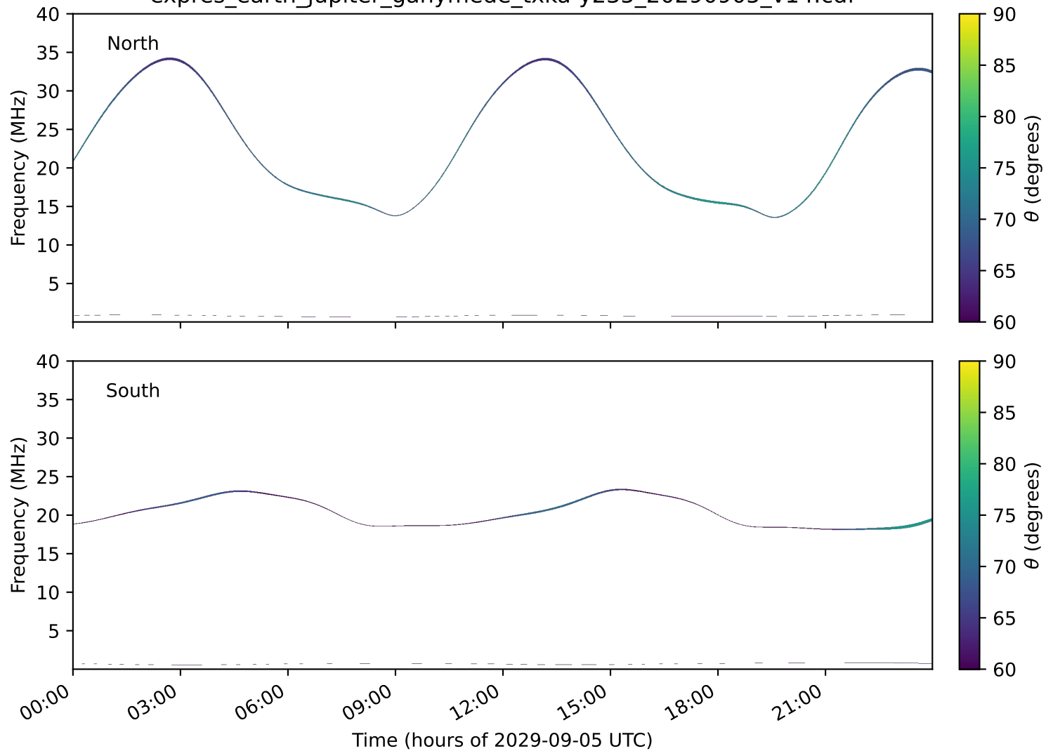
expres_earth_jupiter_ganymede_txka-y235_20290905_v14.cdf
