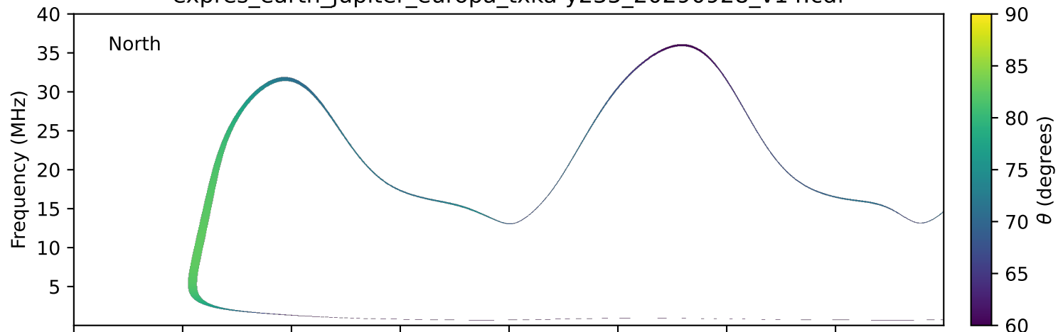
expres_earth_jupiter_europa_txka-y235_20290928_v14.cdf
