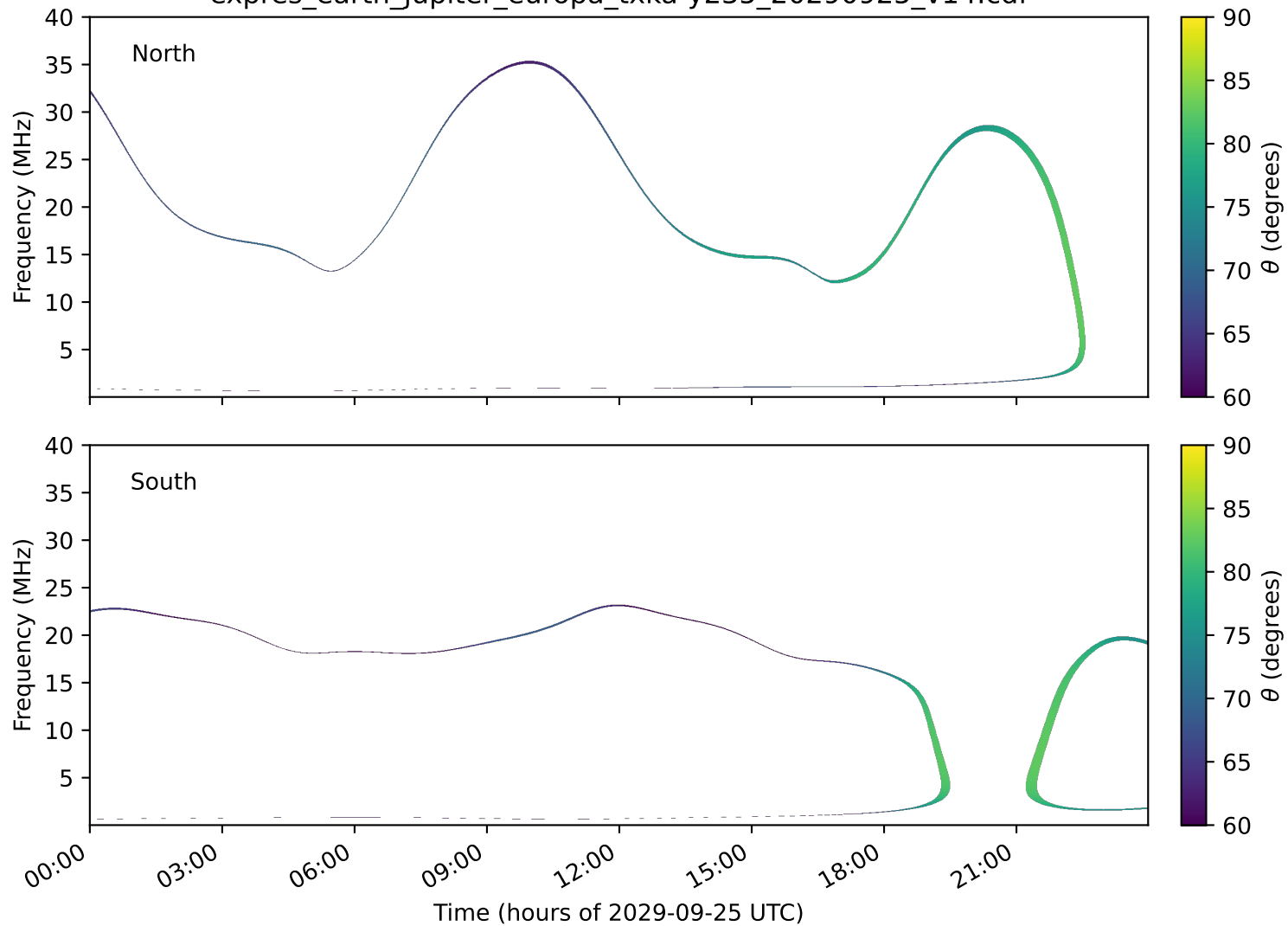
expres_earth_jupiter_europa_txka-y235_20290925_v14.cdf
