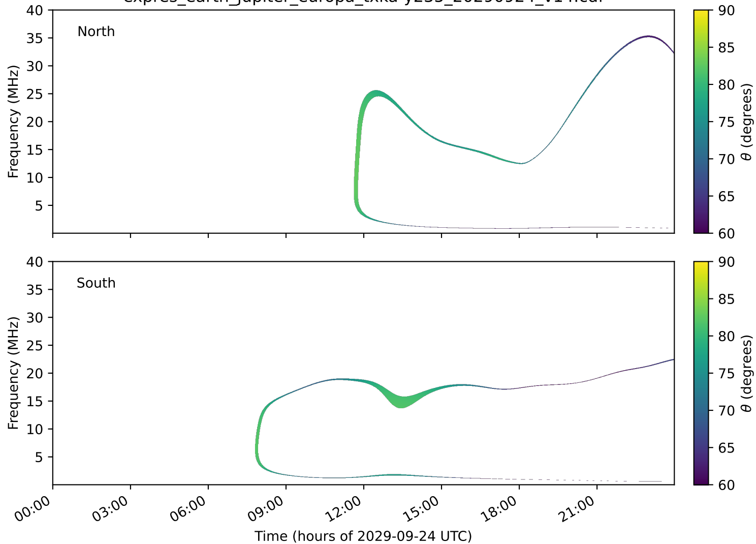
expres_earth_jupiter_europa_txka-y235_20290924_v14.cdf
