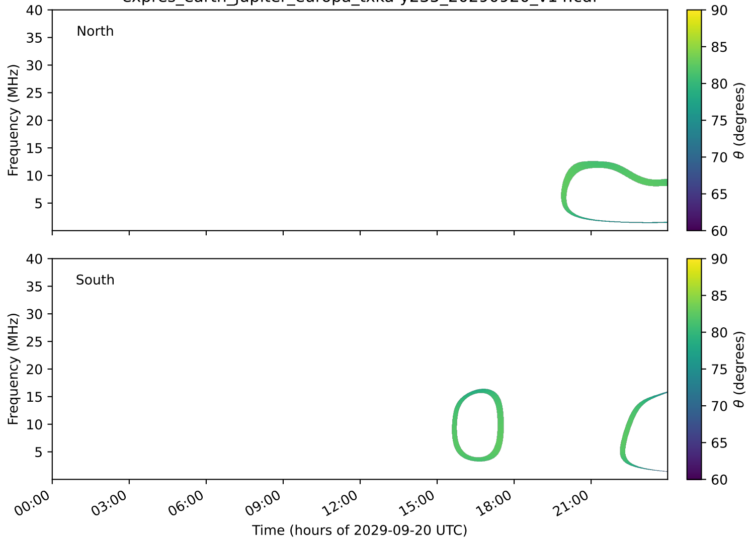
expres_earth_jupiter_europa_txka-y235_20290920_v14.cdf
