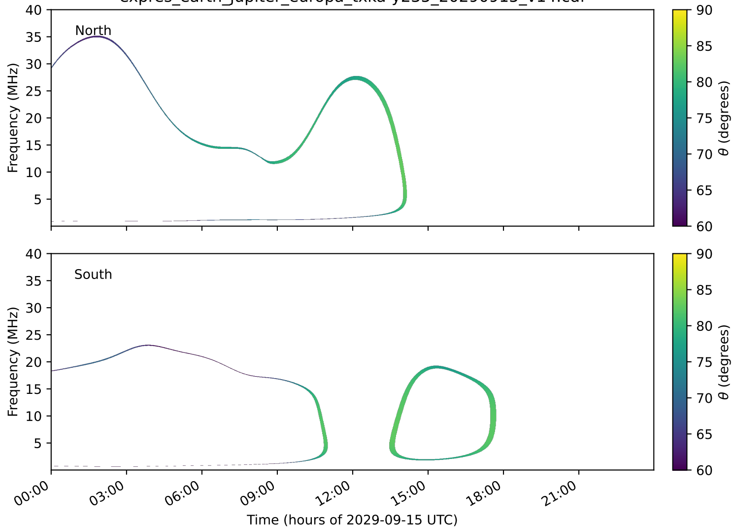
expres_earth_jupiter_europa_txka-y235_20290915_v14.cdf
