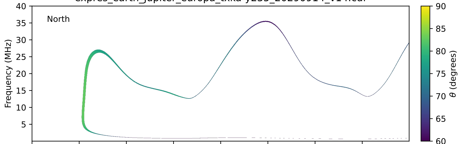
expres_earth_jupiter_europa_txka-y235_20290914_v14.cdf
