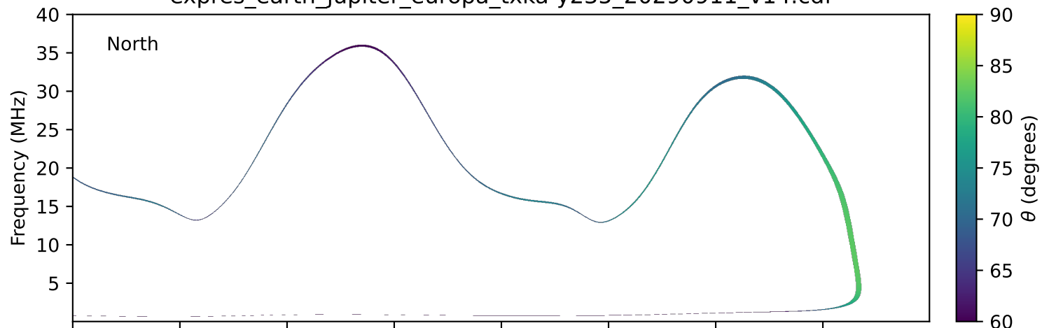
expres_earth_jupiter_europa_txka-y235_20290911_v14.cdf
