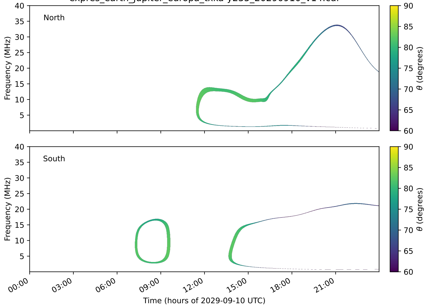
expres_earth_jupiter_europa_txka-y235_20290910_v14.cdf
