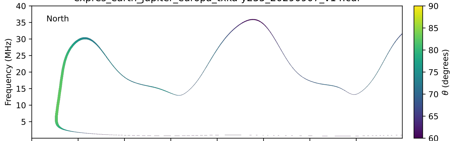
expres_earth_jupiter_europa_txka-y235_20290907_v14.cdf
