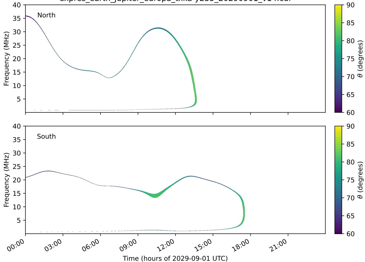
expres_earth_jupiter_europa_txka-y235_20290901_v14.cdf
