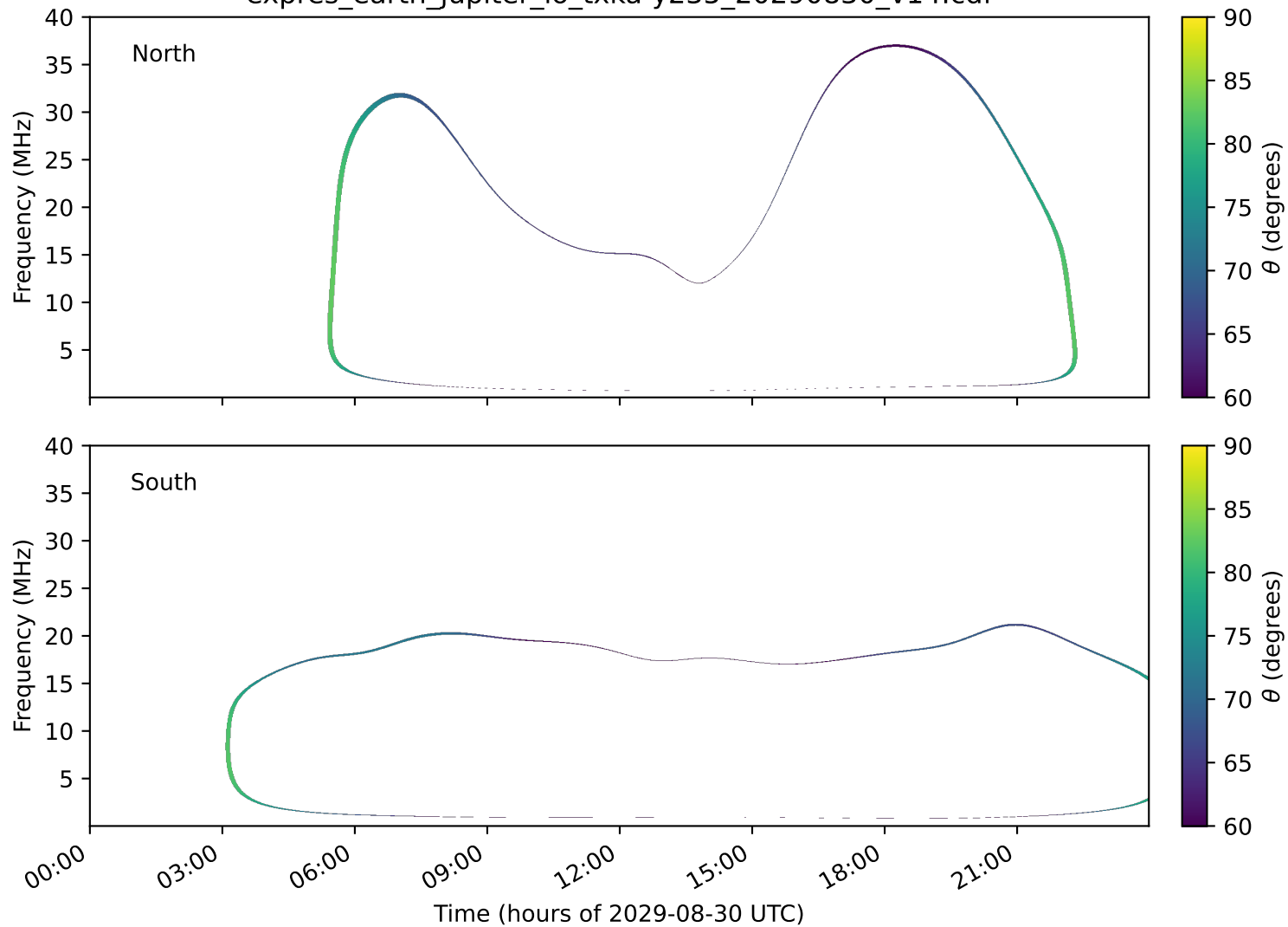
expres_earth_jupiter_io_txka-y235_20290830_v14.cdf
