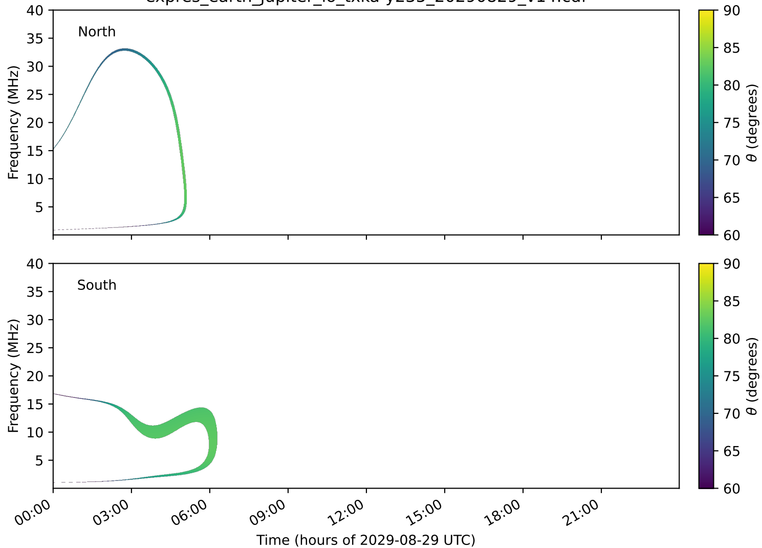
expres_earth_jupiter_io_txka-y235_20290829_v14.cdf
