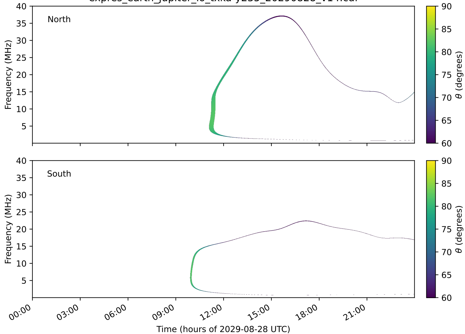
expres_earth_jupiter_io_txka-y235_20290828_v14.cdf
