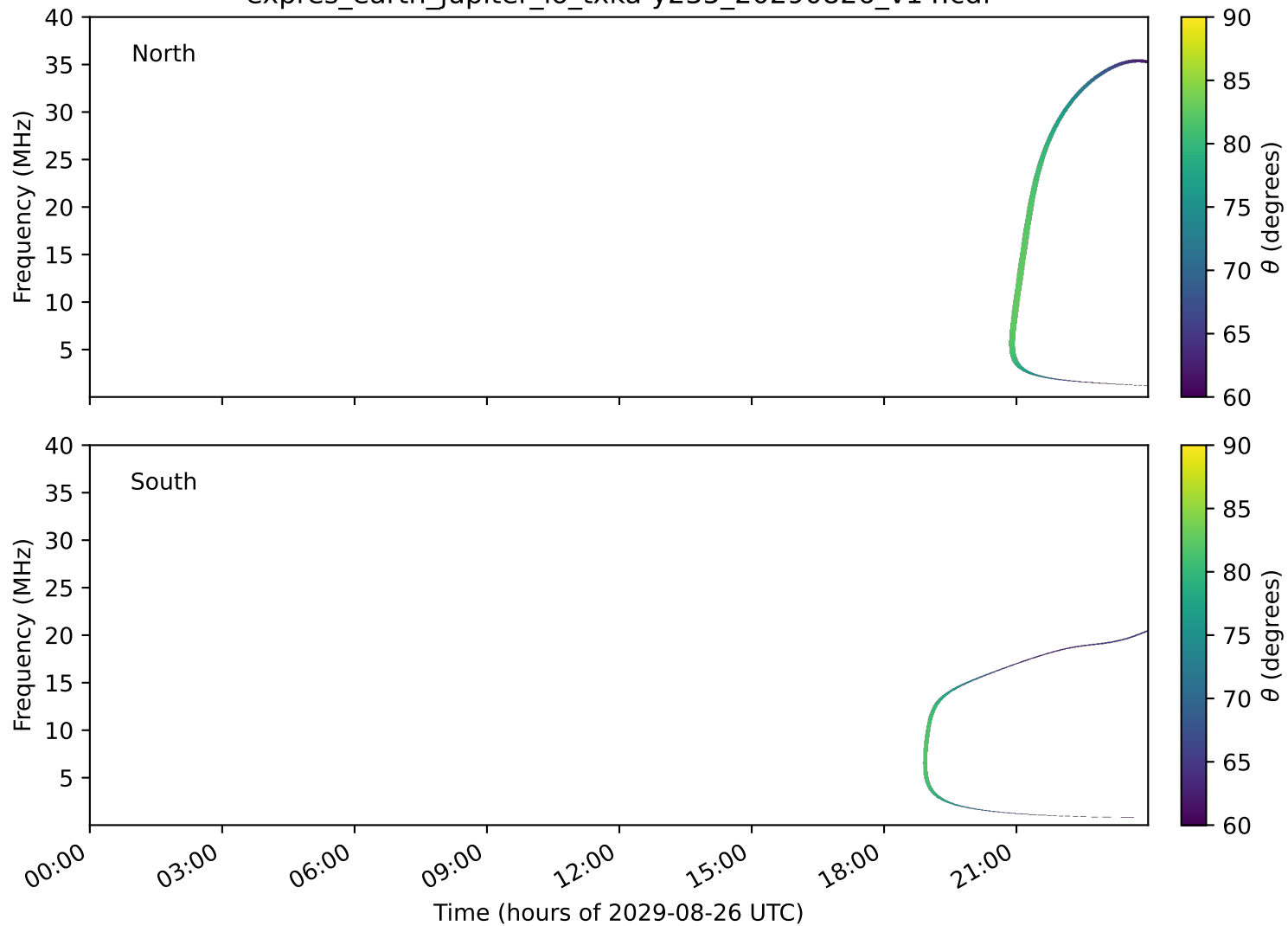
expres_earth_jupiter_io_txka-y235_20290826_v14.cdf
