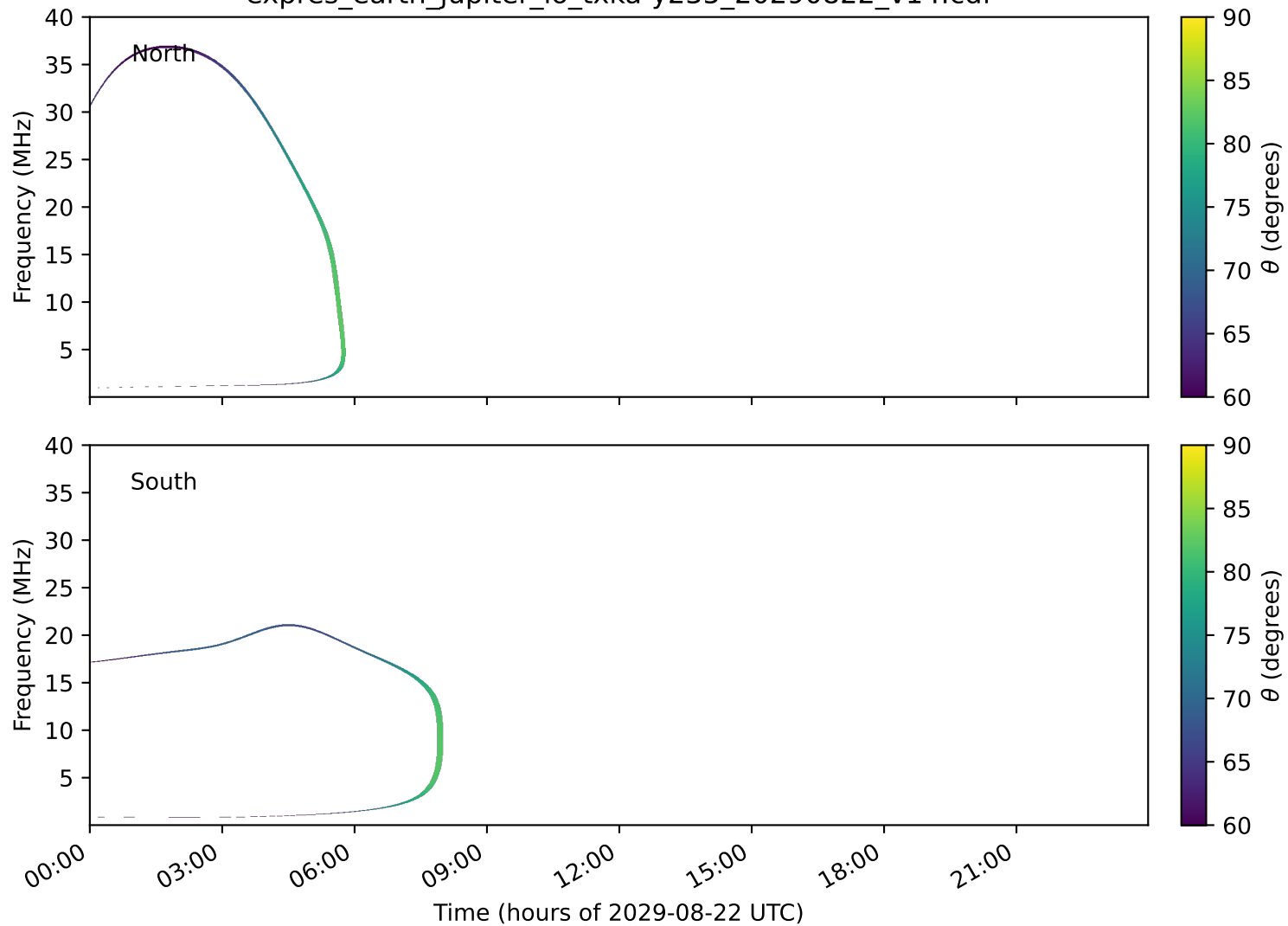
expres_earth_jupiter_io_txka-y235_20290822_v14.cdf
