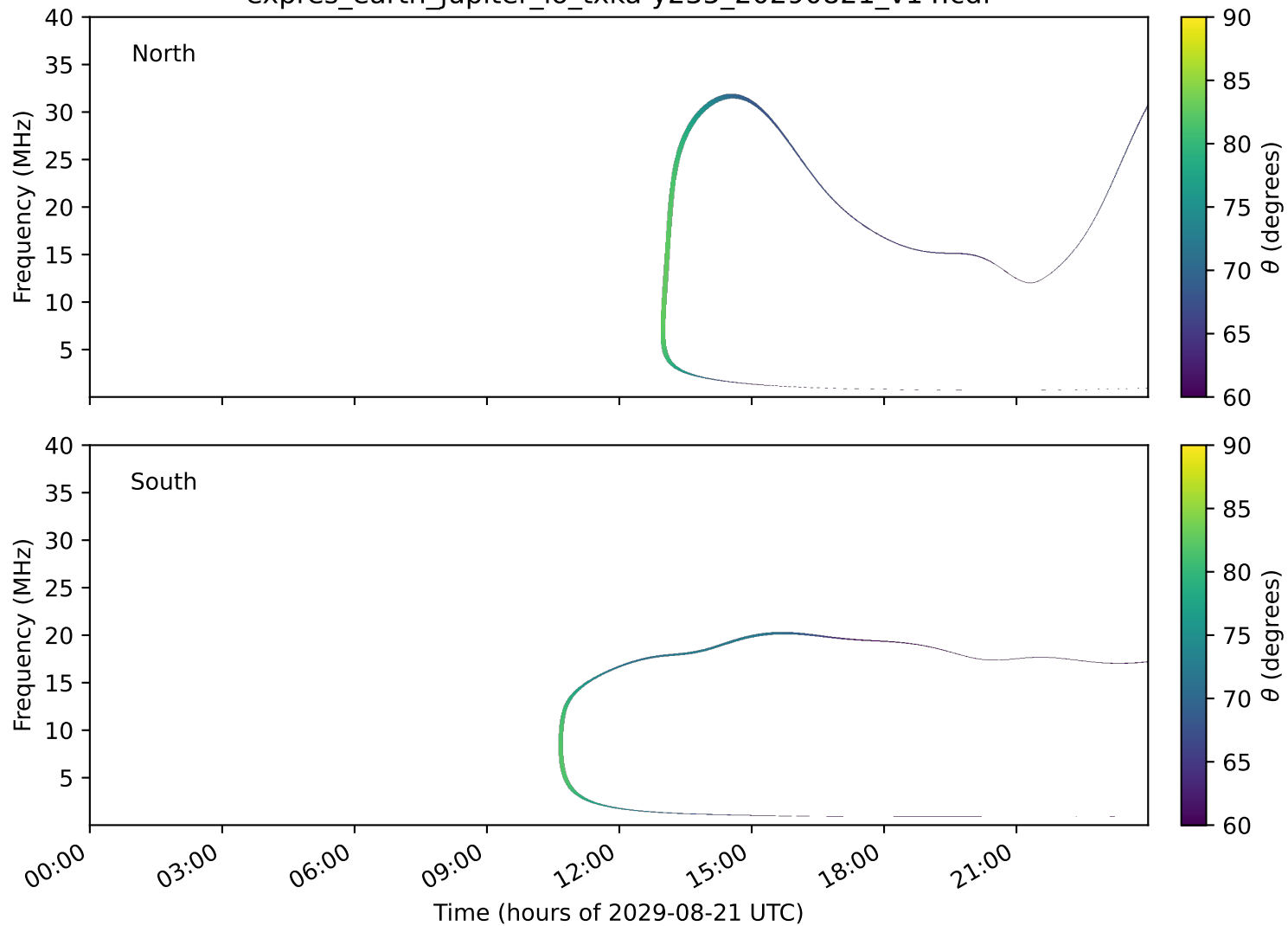
expres_earth_jupiter_io_txka-y235_20290821_v14.cdf
