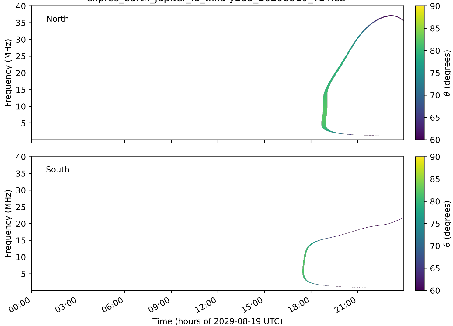
expres_earth_jupiter_io_txka-y235_20290819_v14.cdf
