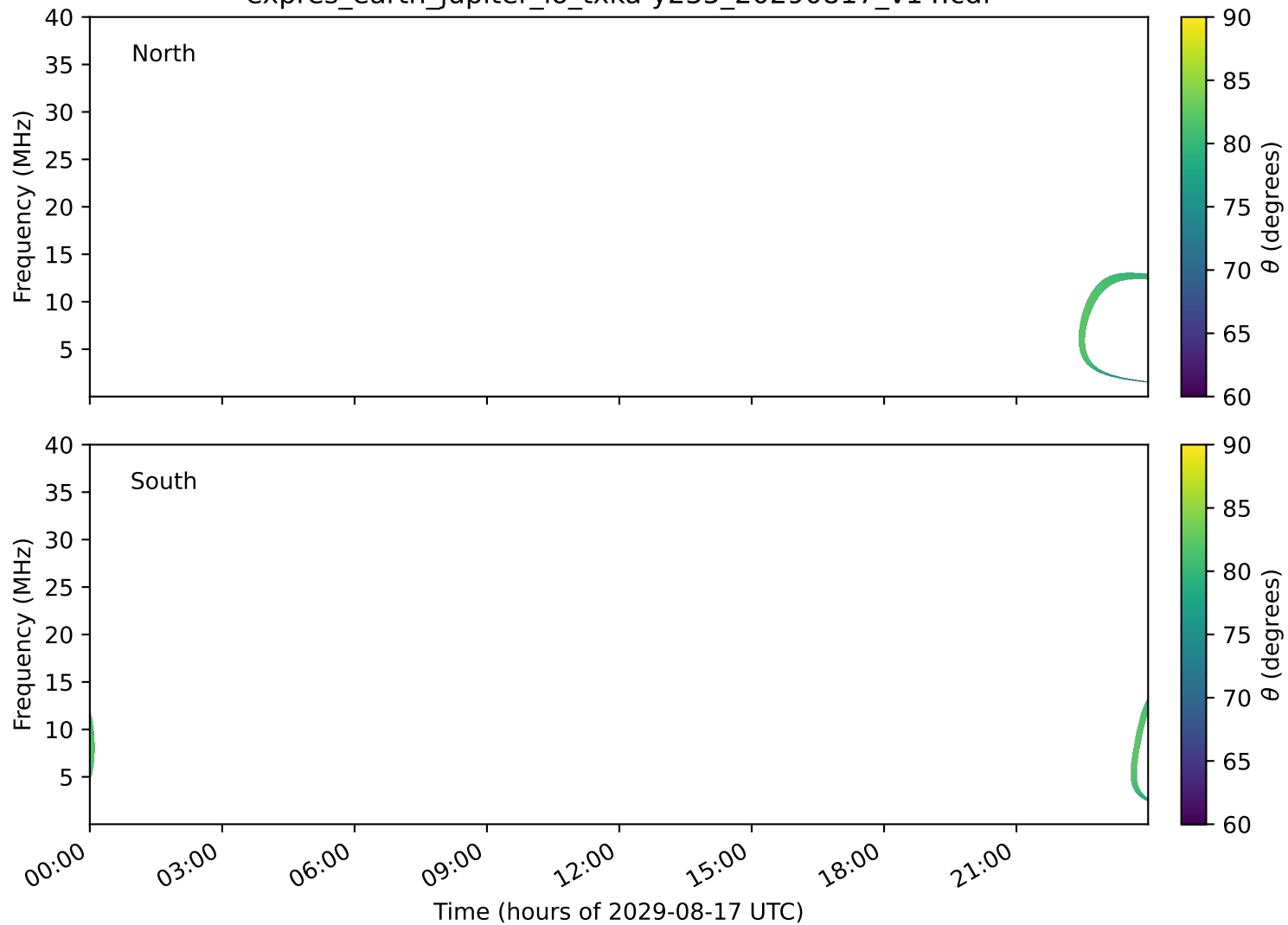
expres_earth_jupiter_io_txka-y235_20290817_v14.cdf
