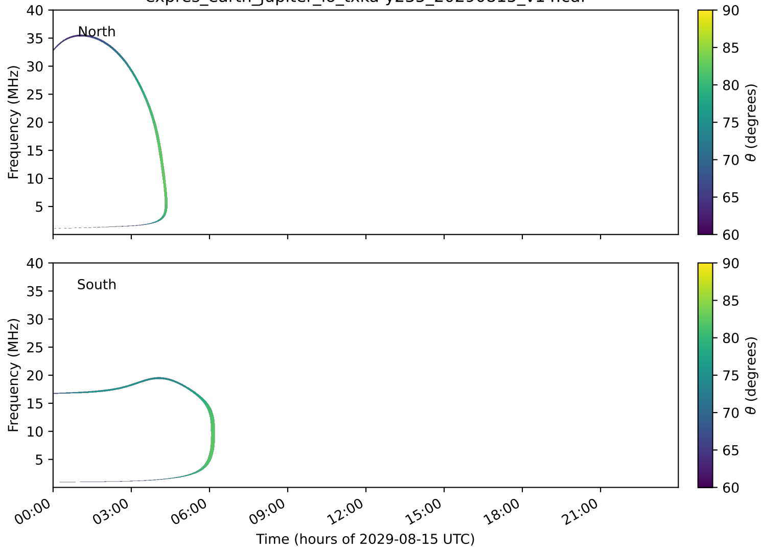
expres_earth_jupiter_io_txka-y235_20290815_v14.cdf
