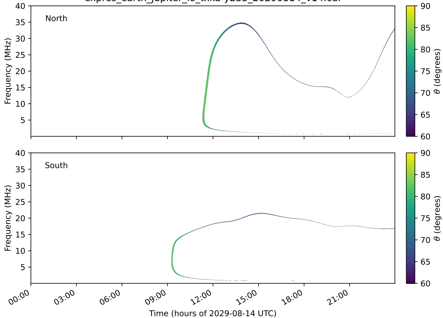
expres_earth_jupiter_io_txka-y235_20290814_v14.cdf
