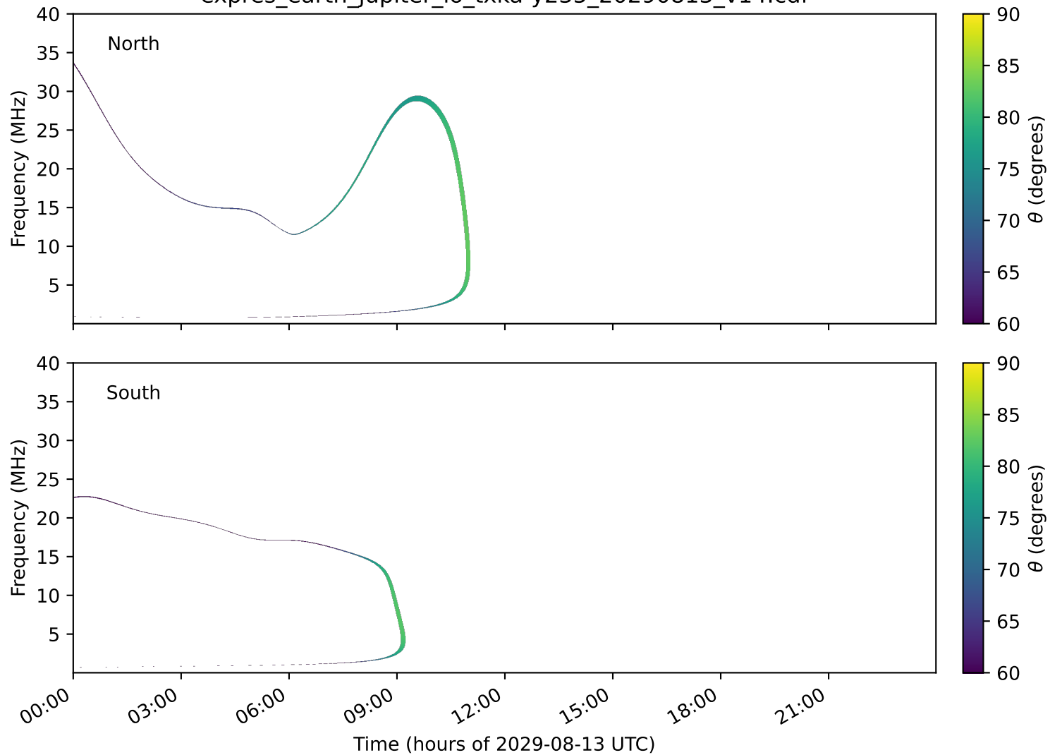
expres_earth_jupiter_io_txka-y235_20290813_v14.cdf
