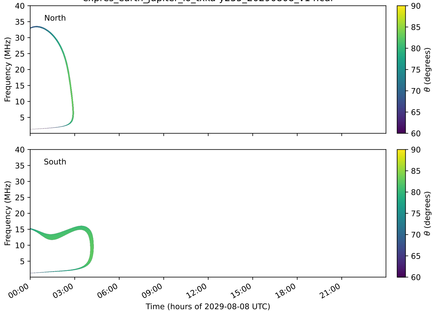
expres_earth_jupiter_io_txka-y235_20290808_v14.cdf
