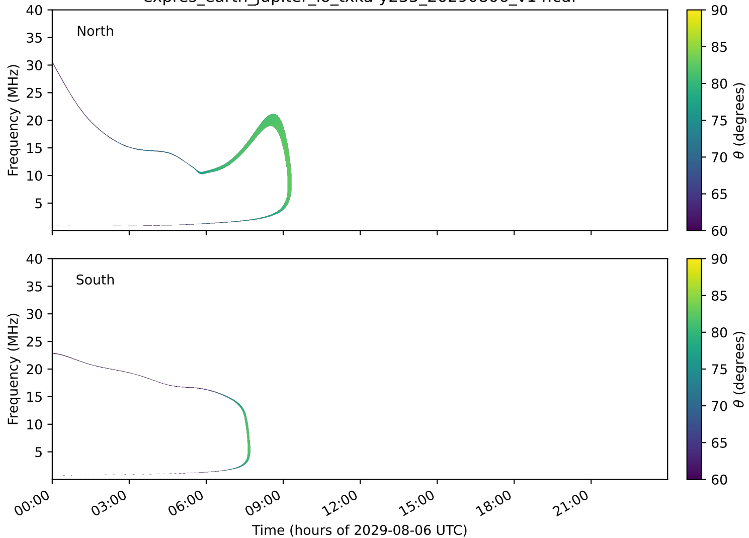
expres_earth_jupiter_io_txka-y235_20290806_v14.cdf
