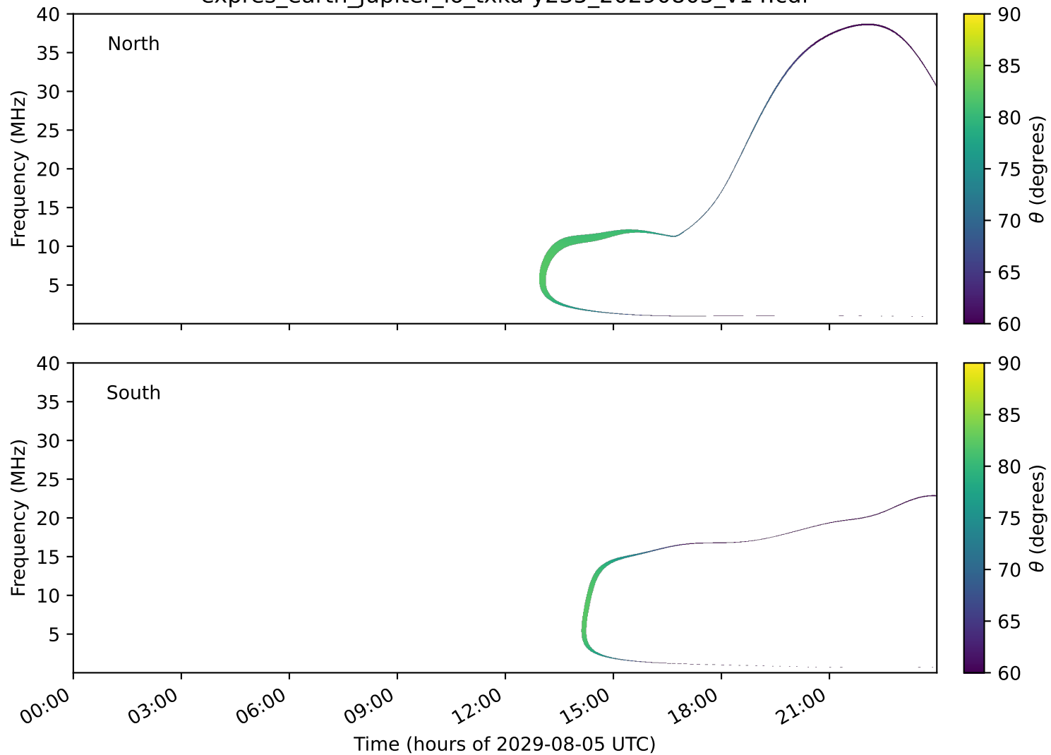
expres_earth_jupiter_io_txka-y235_20290805_v14.cdf
