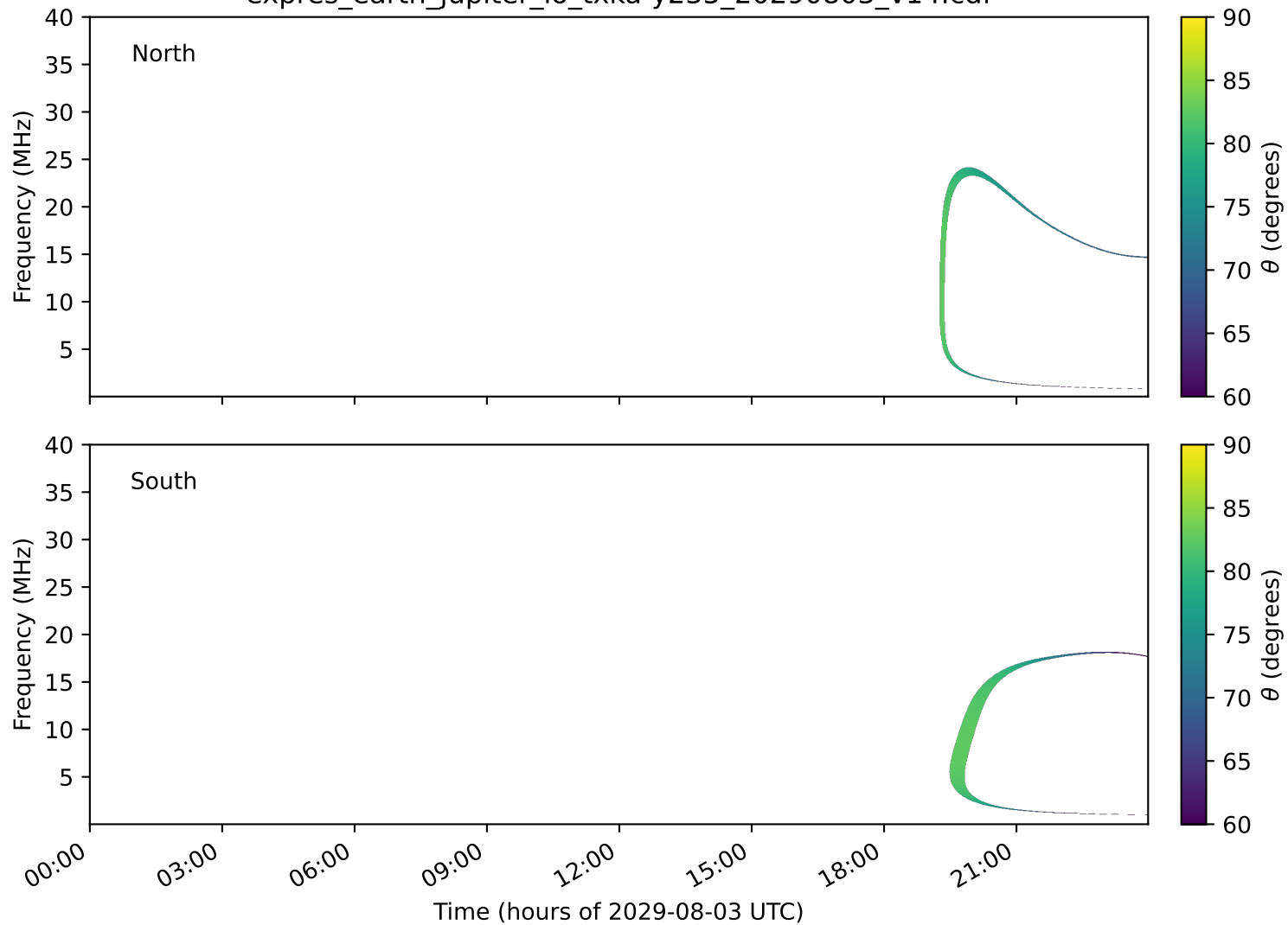
expres_earth_jupiter_io_txka-y235_20290803_v14.cdf
